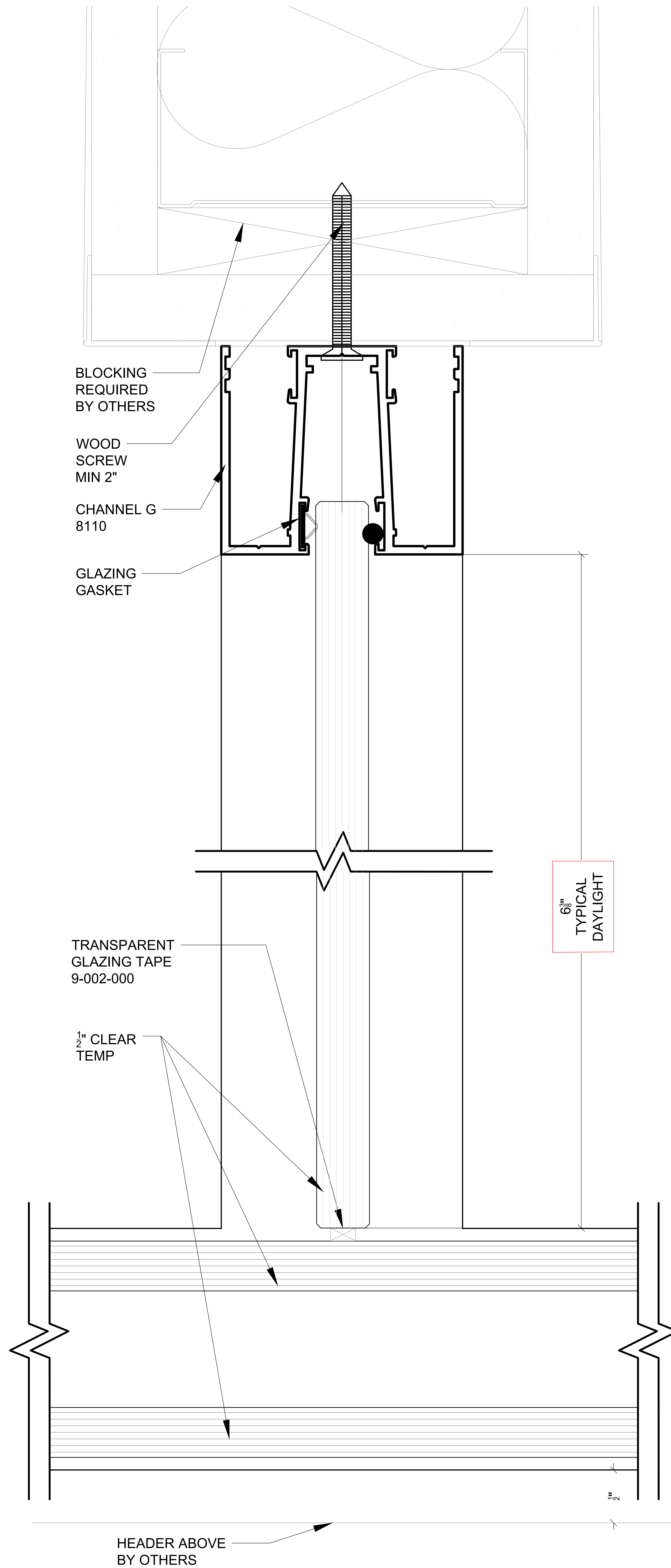
1 3 WAY GLASS CONNECTION DOUBLE GLAZED PANELS 1'-0"=1'-0"
