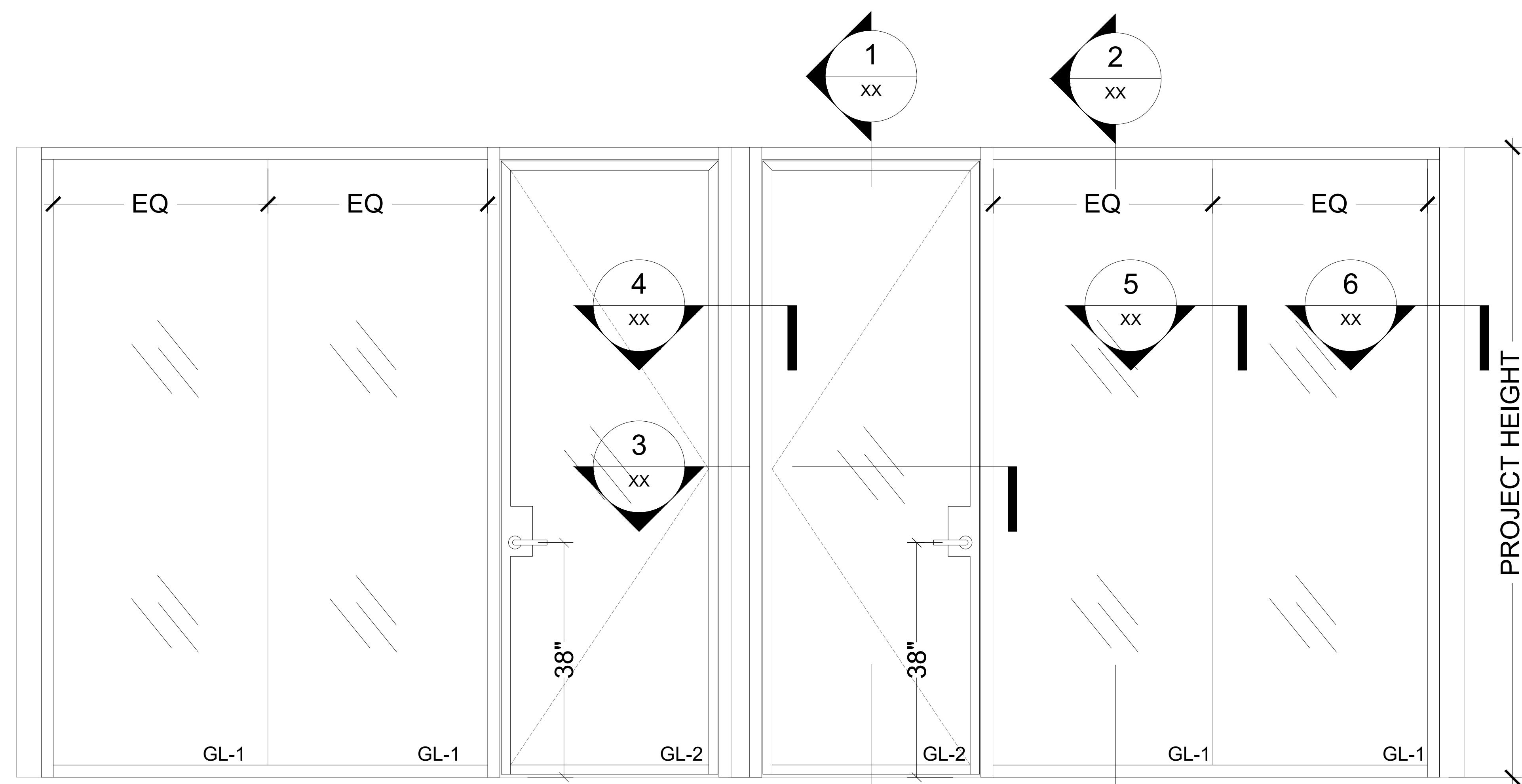
1 ELEVATION 1'-0"=1'-0"
