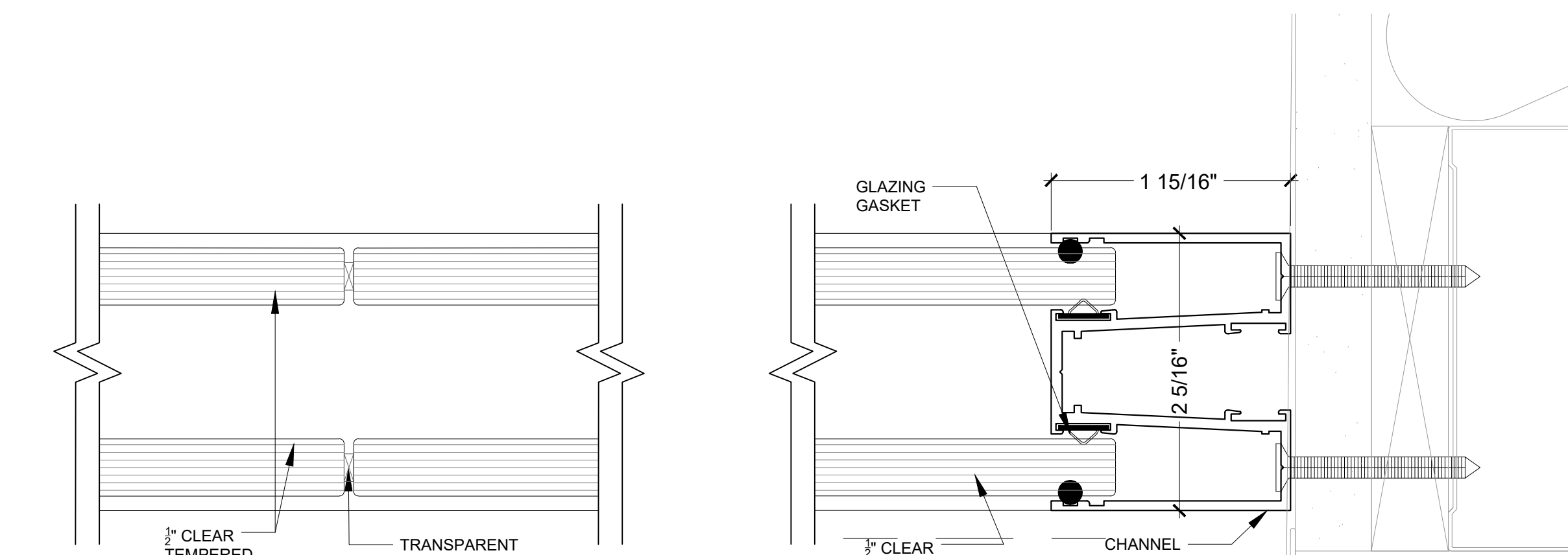
5 GLASS CONNECTION 1'-0"=1'-0"
