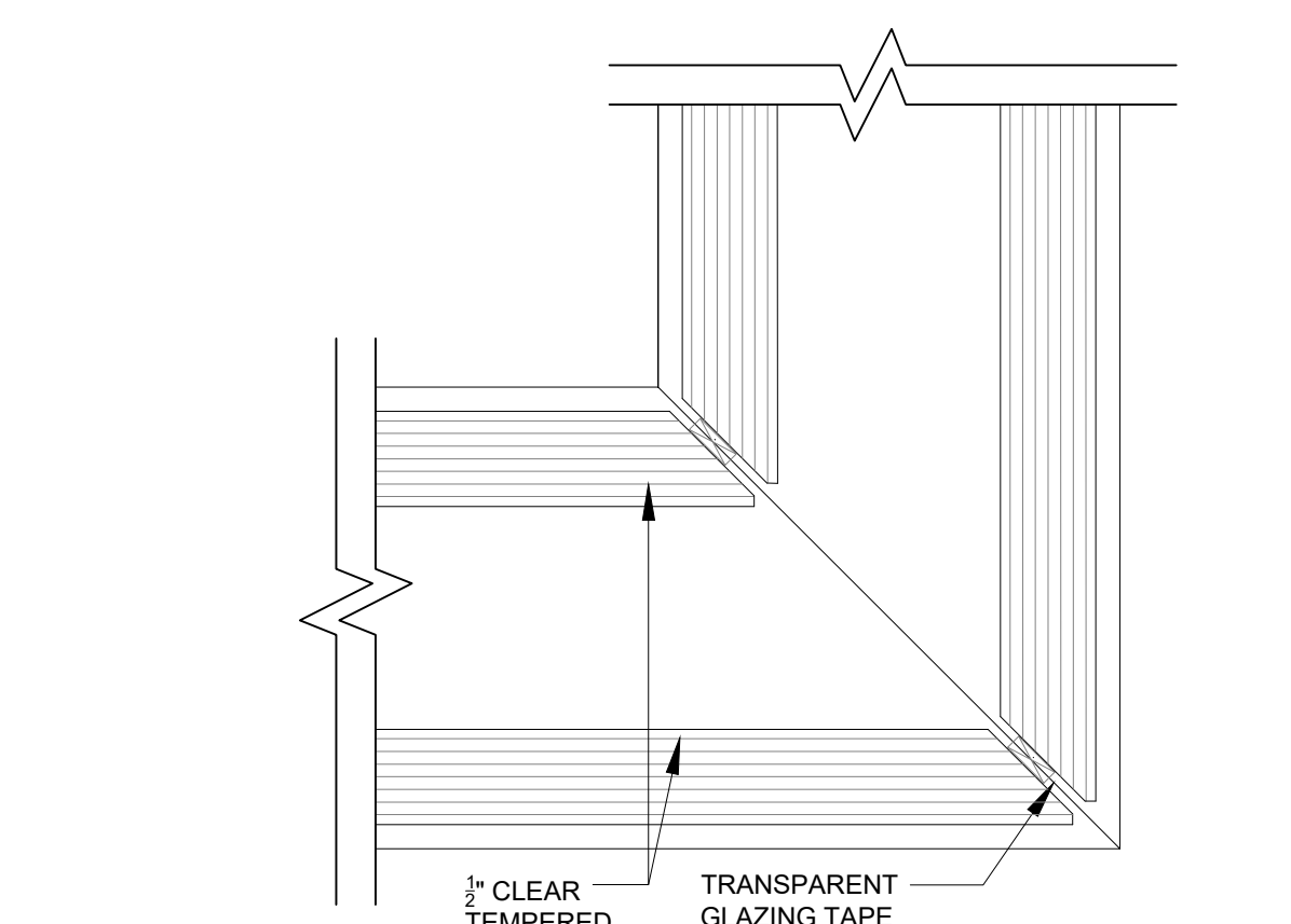
7 GLASS CORNER 1'-0"=1'-0"
