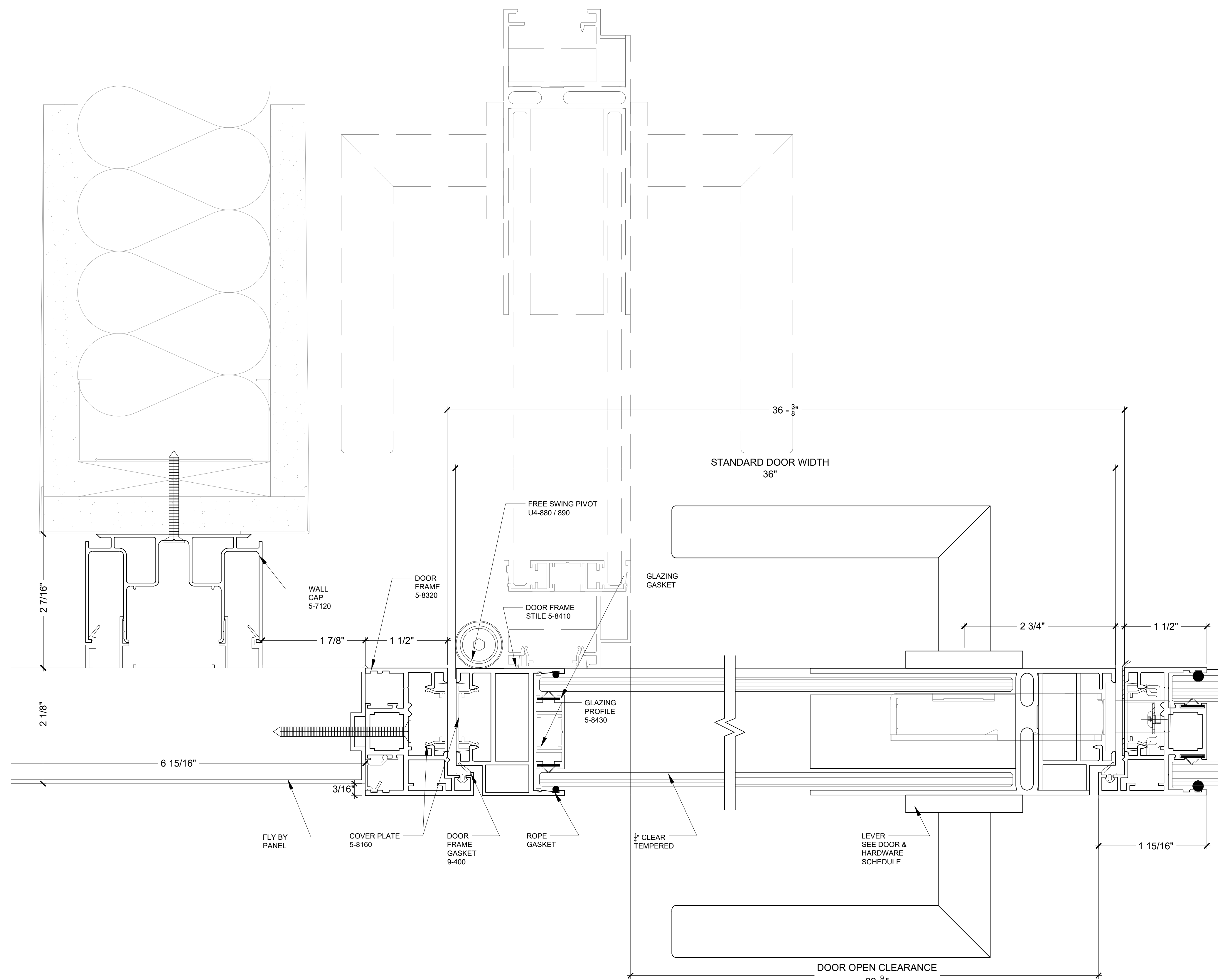
3 FRAMED PIVOT DOOR W/ LEVER HANDLE 1'-0"=1'-0"
